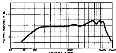
TYPICAL FREQUENCY RESPONSE FIGURE 1
