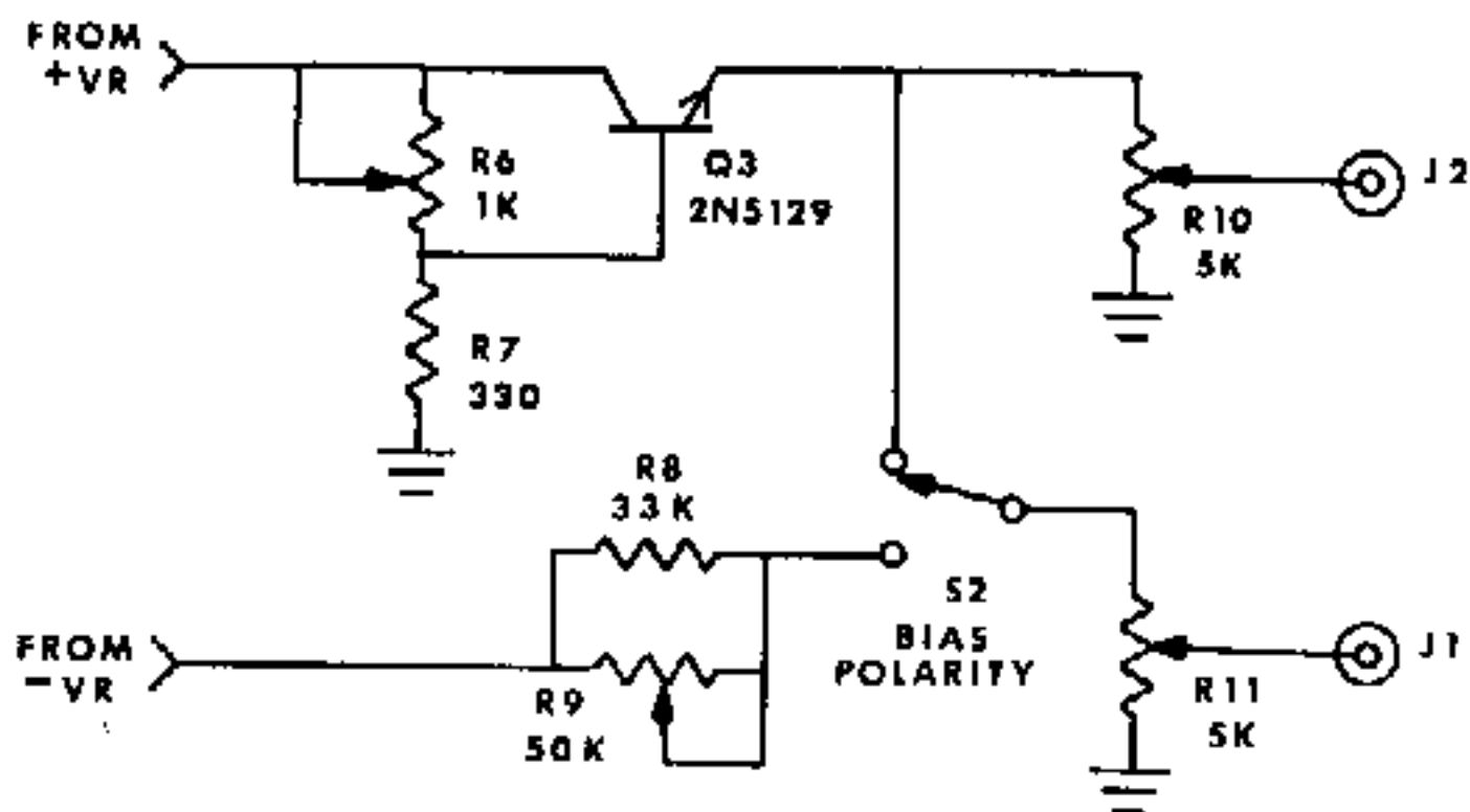
Figure 7 - Schematic diagram
