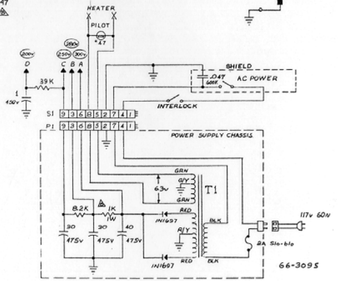
POWER SUPPLY CHASSIS
